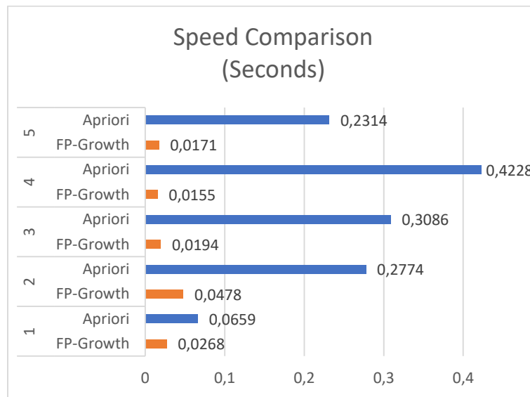
Figure 5. Comparison of Algorithm Processing Speed
