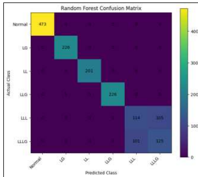
Figure 3. Confusion Matrix of the Random Forest Model
