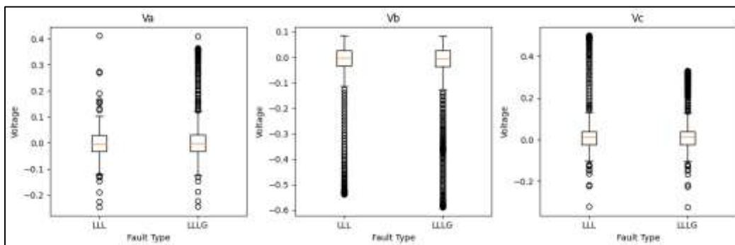
Figure 8. Distribution of Voltage Features for LLL and LLLG Fault Classes
