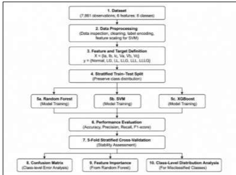
Figure 1. Research Framework for Multiclass Electrical Fault Classification
