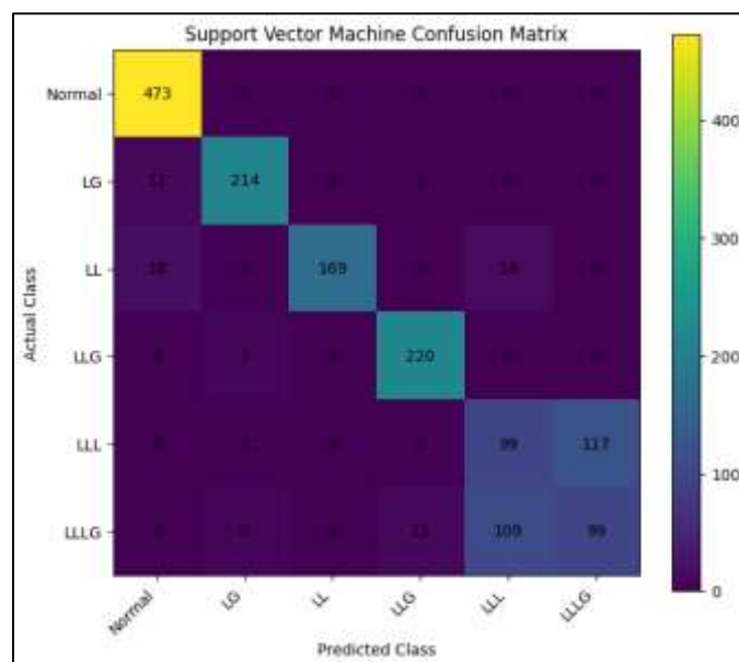
Figure 4. Confusion Matrix of the Support Vector Machine Model
