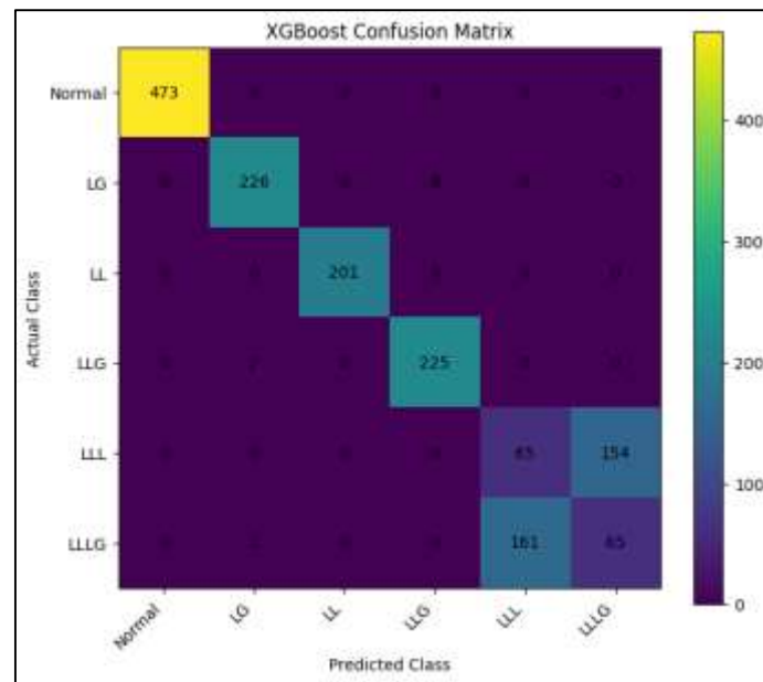
Figure 5. Confusion Matrix of the XGBoost Model
