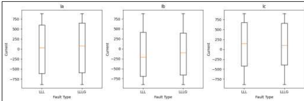
Figure 7. Distribution of Current Features for LLL and LLLG Fault Classes
