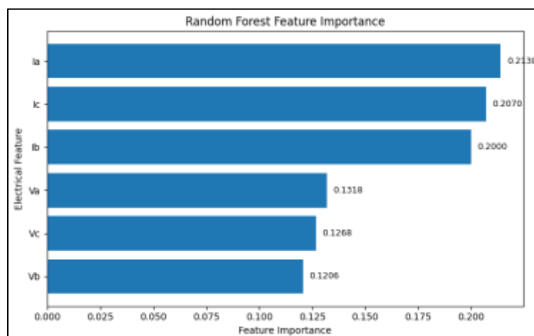
Figure 6. Random Forest Feature Importance
