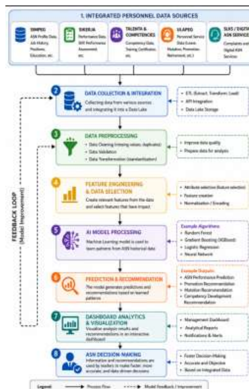
Figure 3. Artificial Intelligence Implementation Flowchart in the Integrated Personnel Information System
